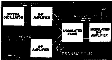
Main sections of a broadcast transmitter.
